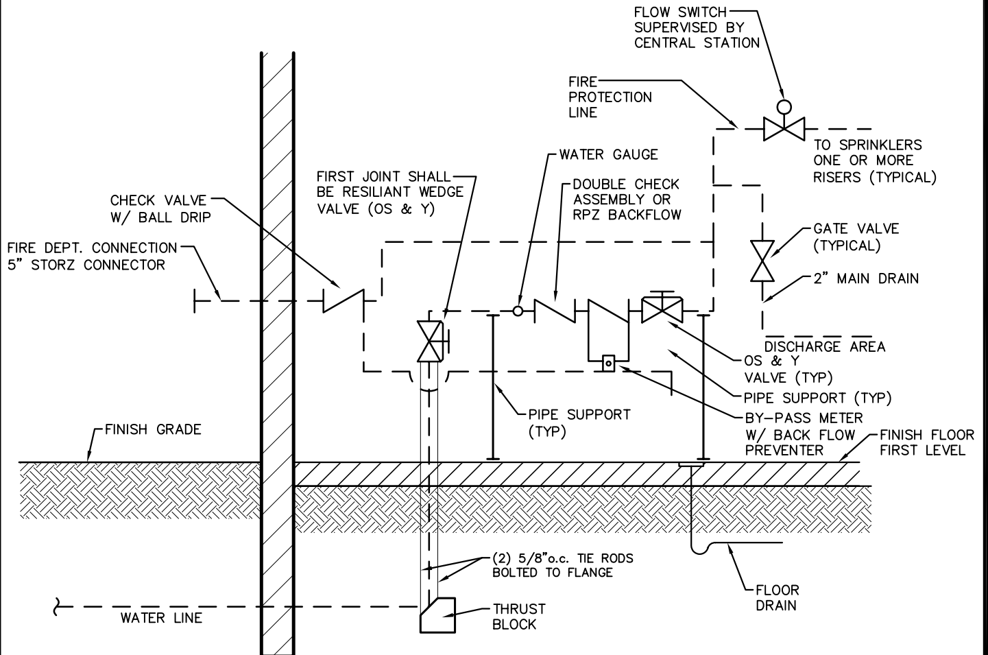
MINIMUM STANDARDS FIRE PROTECTION RISER DIAGRAM N.T.S.
